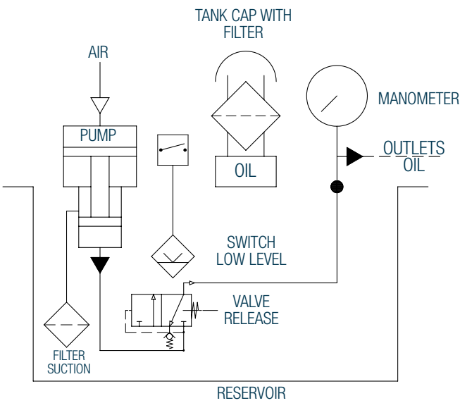
hydraulic layout with pneumatic pump
