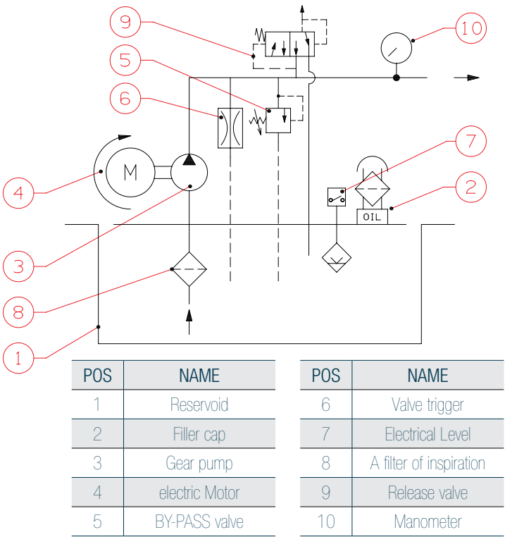
hydraulic layout with electric pump
